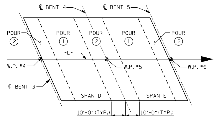
POURING SEQUENCE - SPANS D & E
